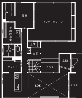
1F
